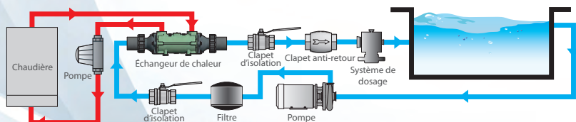
Montage vertical
